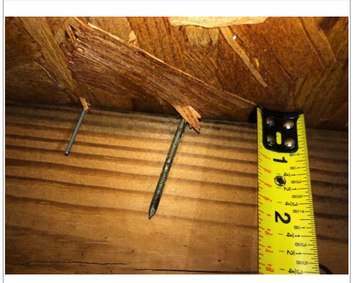
8d Nails
